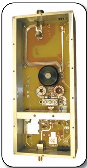
Prototype Class-E transmit amplifier shown here.
