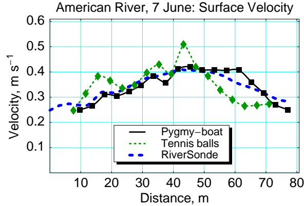
Figure 4: American River velocity profiles for 7 June 2000. Distance is measured across the channel from the bank near the receive antenna. The in-situ measurements were from a flow meter suspended from a small boat about 150 m from the radar (Pygmy-boat), and from optical tracking of floating tennis balls (Tennis balls).
