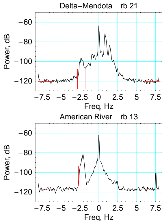
Figure 2: Spectrum of received energy at the Delta-Mendota Canal on 5 June 2000 (top) and at the American River on 7 June 2000 (bottom). The waves are moving predominately toward the radar at the canal and away from the radar at the river. The short red lines indicate the estimated noise level and the region of the spectrum selected for MUSIC direction finding.
