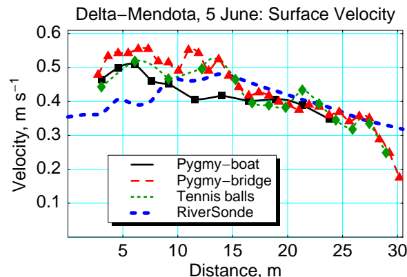
Figure 3: Delta-Mendota velocity profiles for 5 June 2000. Distance is measured across the channel from the bank near the receive antenna. The in-situ measurements were from a flow meter suspended from a small boat about 60 m from the bridge (Pygmy-boat) or with the boat tethered to the bridge (Pygmy-bridge), and from optical tracking of floating tennis balls (Tennis balls). The RiverSonde measurements are shown as a thick dashed blue line.
