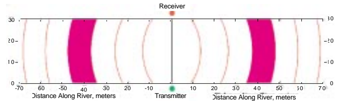
Figure 1: Bistatic scattering geometry. Transmitter and receiver are on opposite sides of a river or canal. Contours of constant time delay are ellipses, and velocity is measured in a direction perpendicular to the ellipses. A scattering cell at 40 m range is highlighted.
